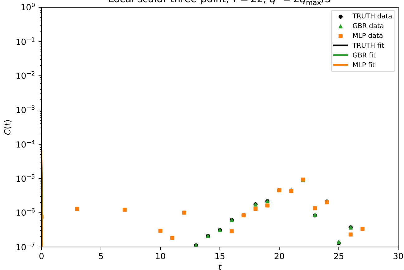
Local scalar three-point, T = 22 , q^2 = 2q_{\max}^2/3
